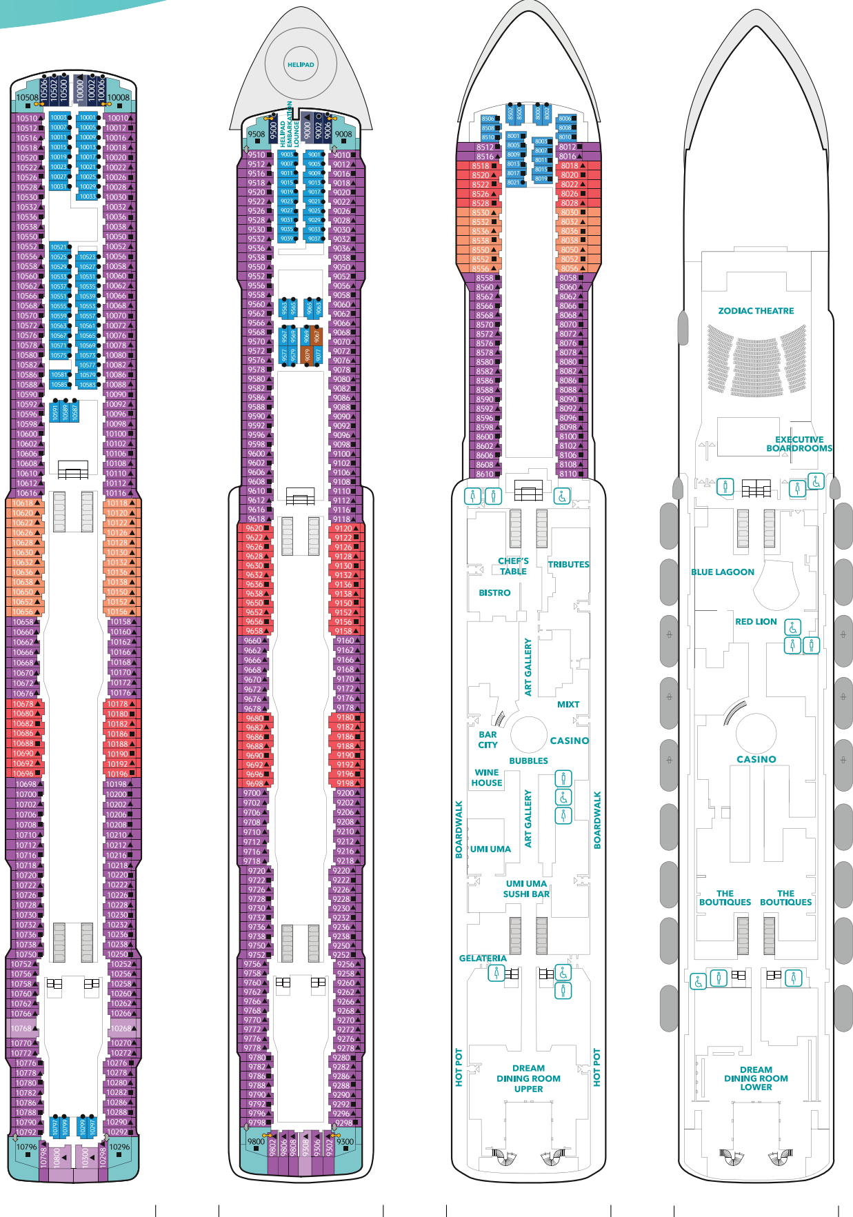
DECK 10
